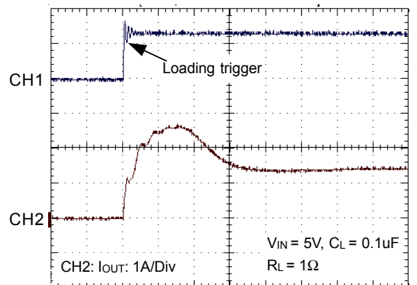
Time (5us/Div)
